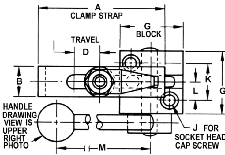
TOP VIEW WITH HANDLE DRAWING FOR FLANGE NUT STYLE
